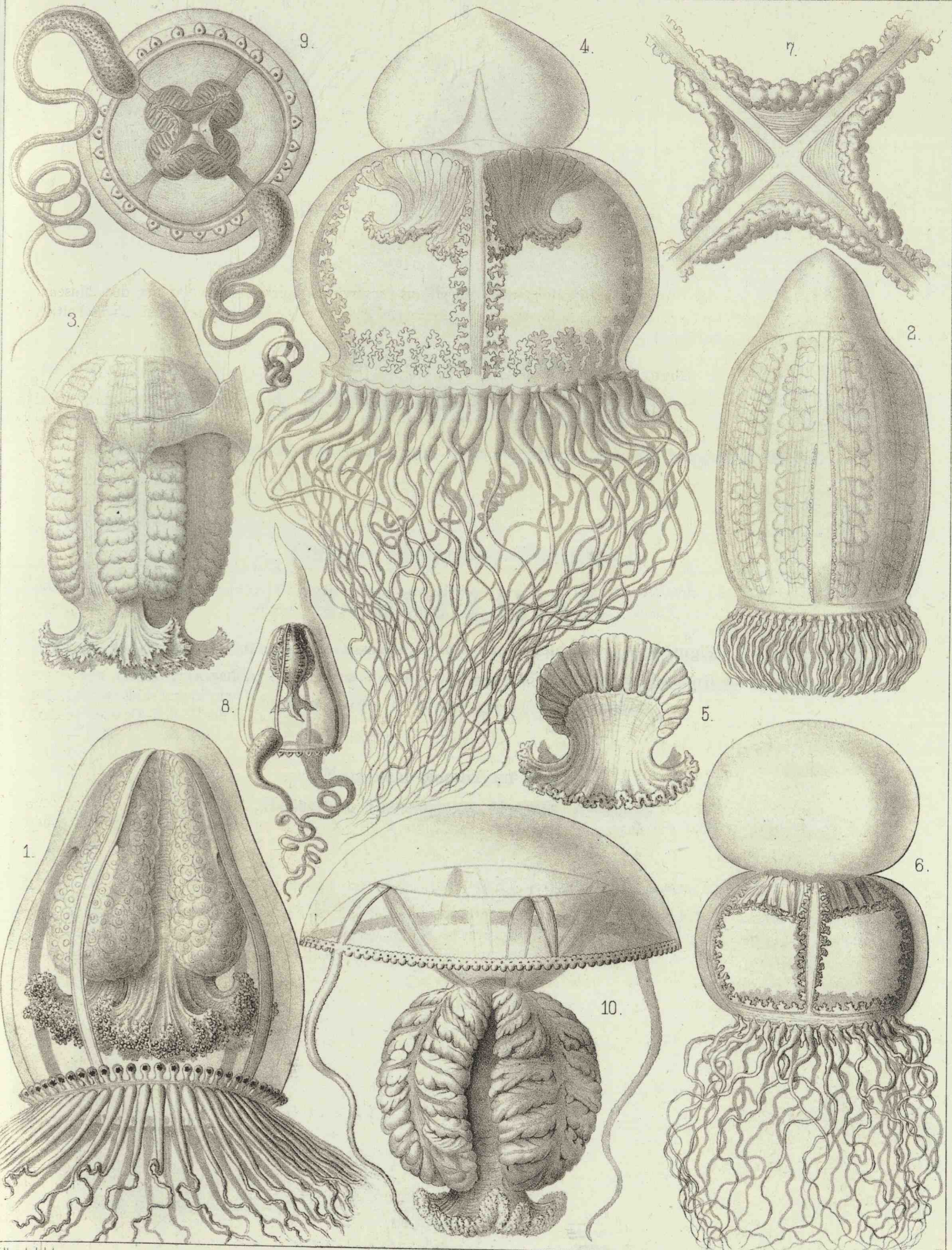
1. CONIS, 2, 3. TURRIS, 4-7. CATABLEMA, 8, 9. DINEMA, 10. STOMOTOCA.
