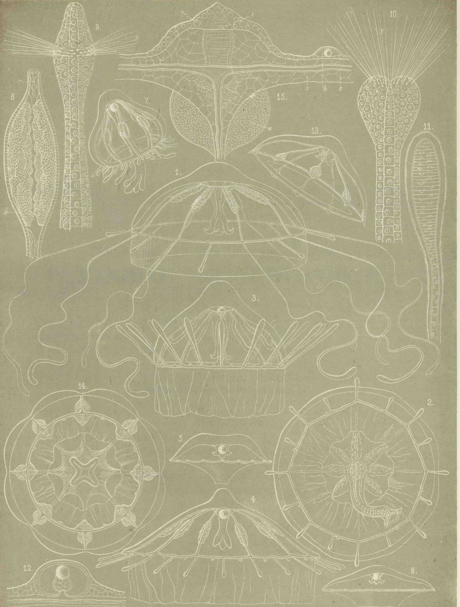
1-3 RHOPALONEMA, 3-12 TRACHYNEMA, 13-15 SMINTHONEMA
