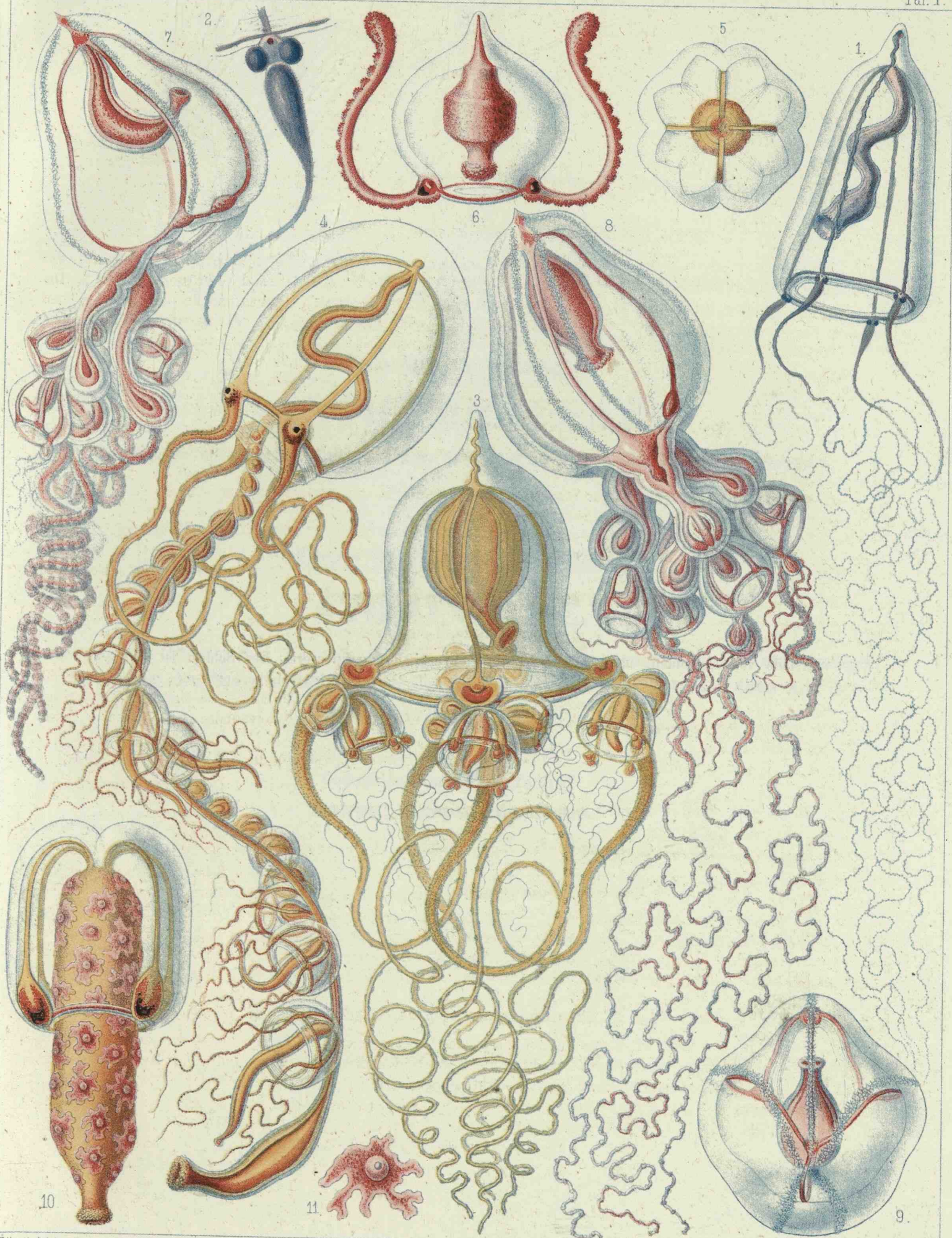
1-3. CODONIUM, 4. 5. SARSIA, 6. DICOTONIUM, 7-9 AMPHICODON, 10. 11. AMALTHAEA.
