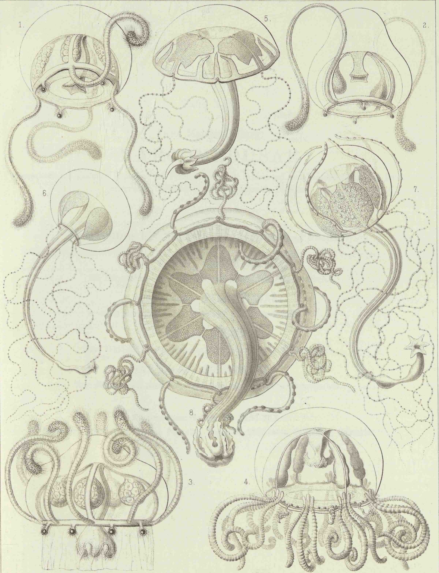
1. PETASUS, 2. DIPETANUS, 3. PETASATA, 4. GOSSEA, 5. GLOSSOCODON, 6. LIRIOPE, 7. GERYONES, 8. CARMARIS.
