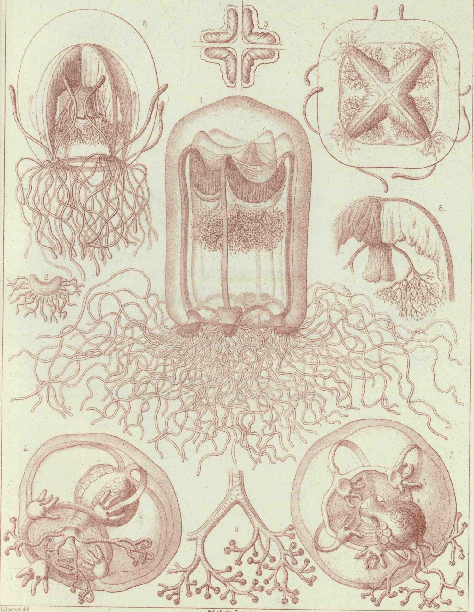
1-3 MARGELIS, 4-5 HIPPOCRENE, 6-9 NEMOPSIS.
