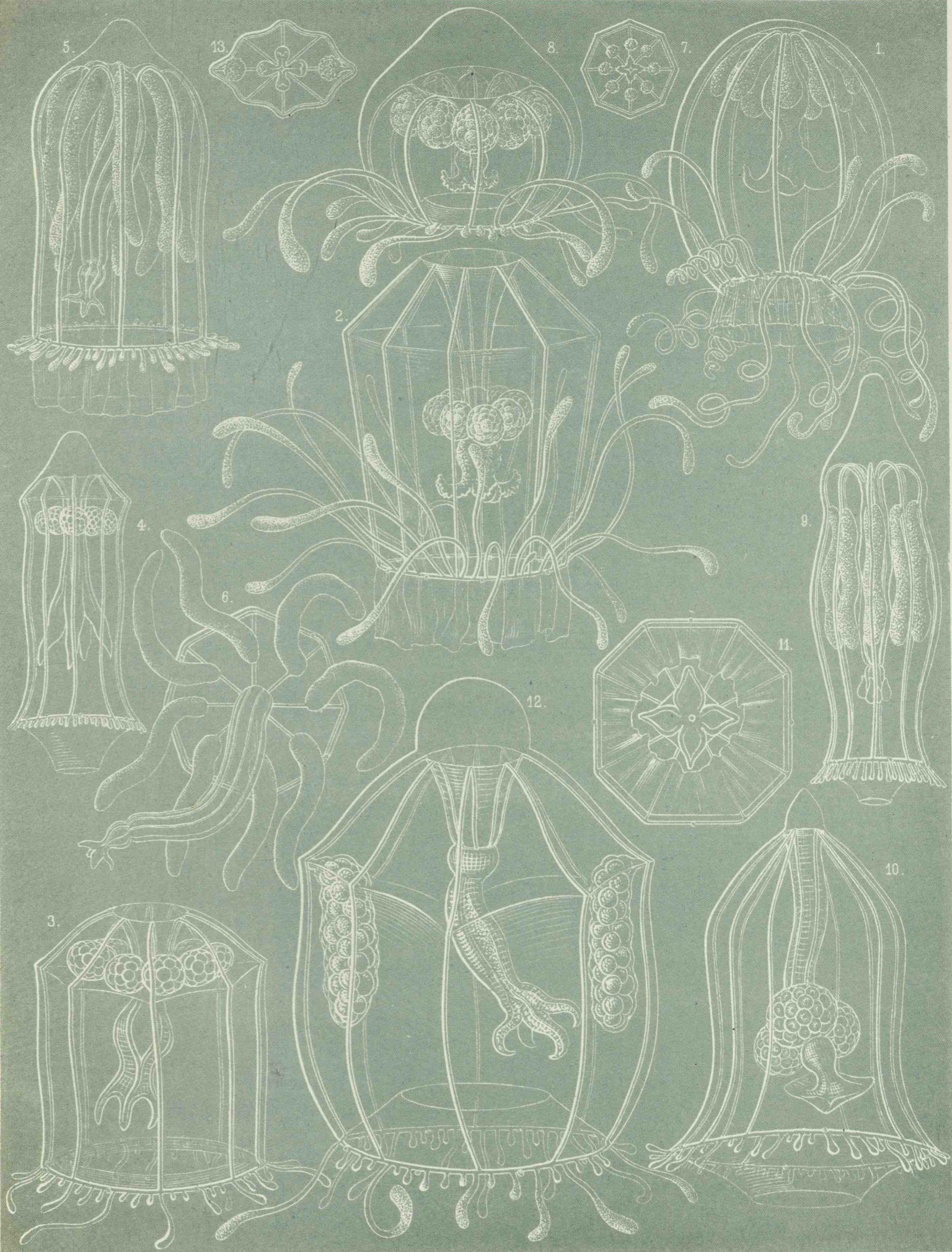
1 AGLAURELLA, 2-4 AGLAURA, 5-8 CIRCCELLA, 9 CIRCETTA, 10-11 STAURAGLAURA, 12-13 PERSA
