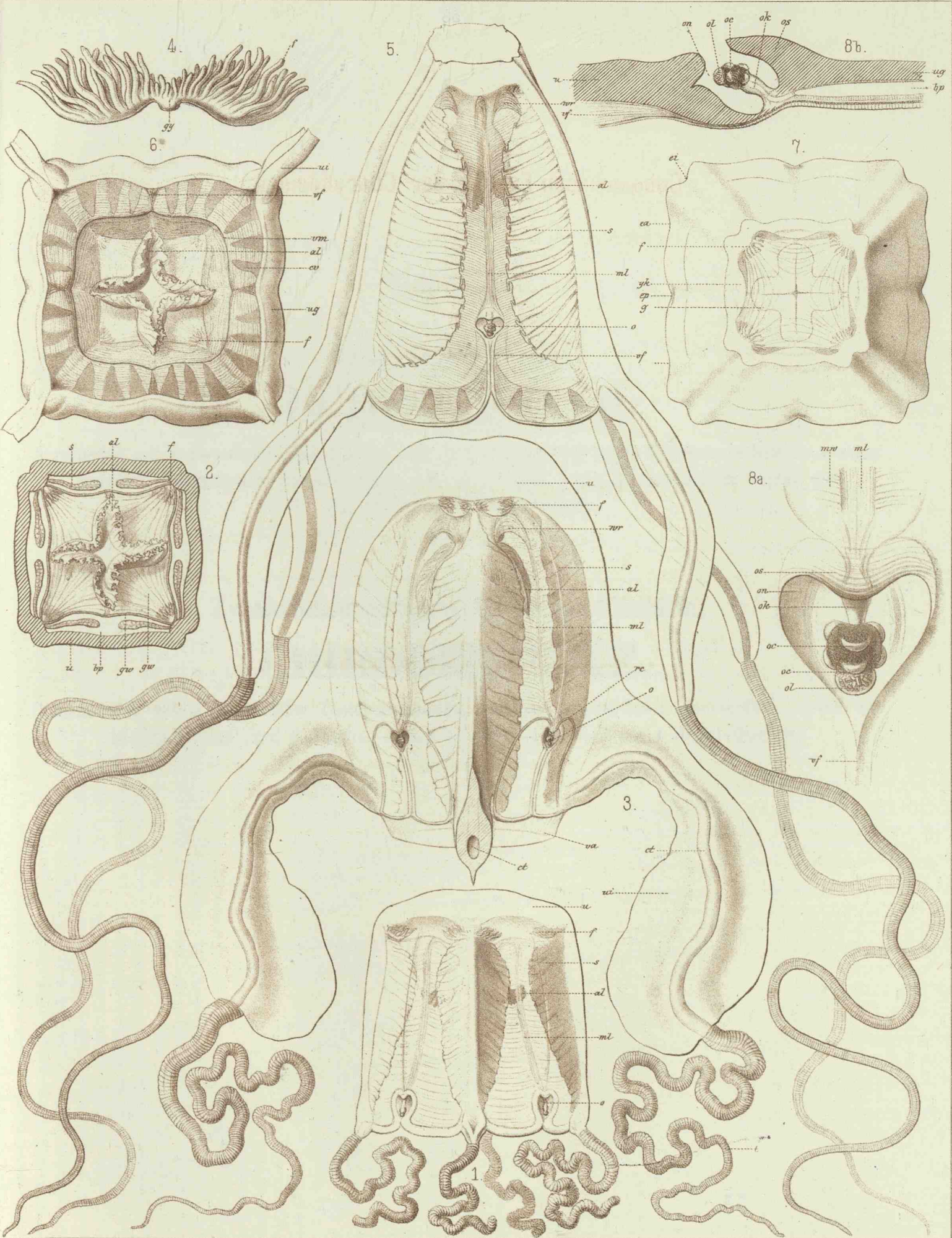
1. 2. PROCHARAGMA, 3. 4. PROCHARYBDIS, 5.-8. CHARYBDEA.
