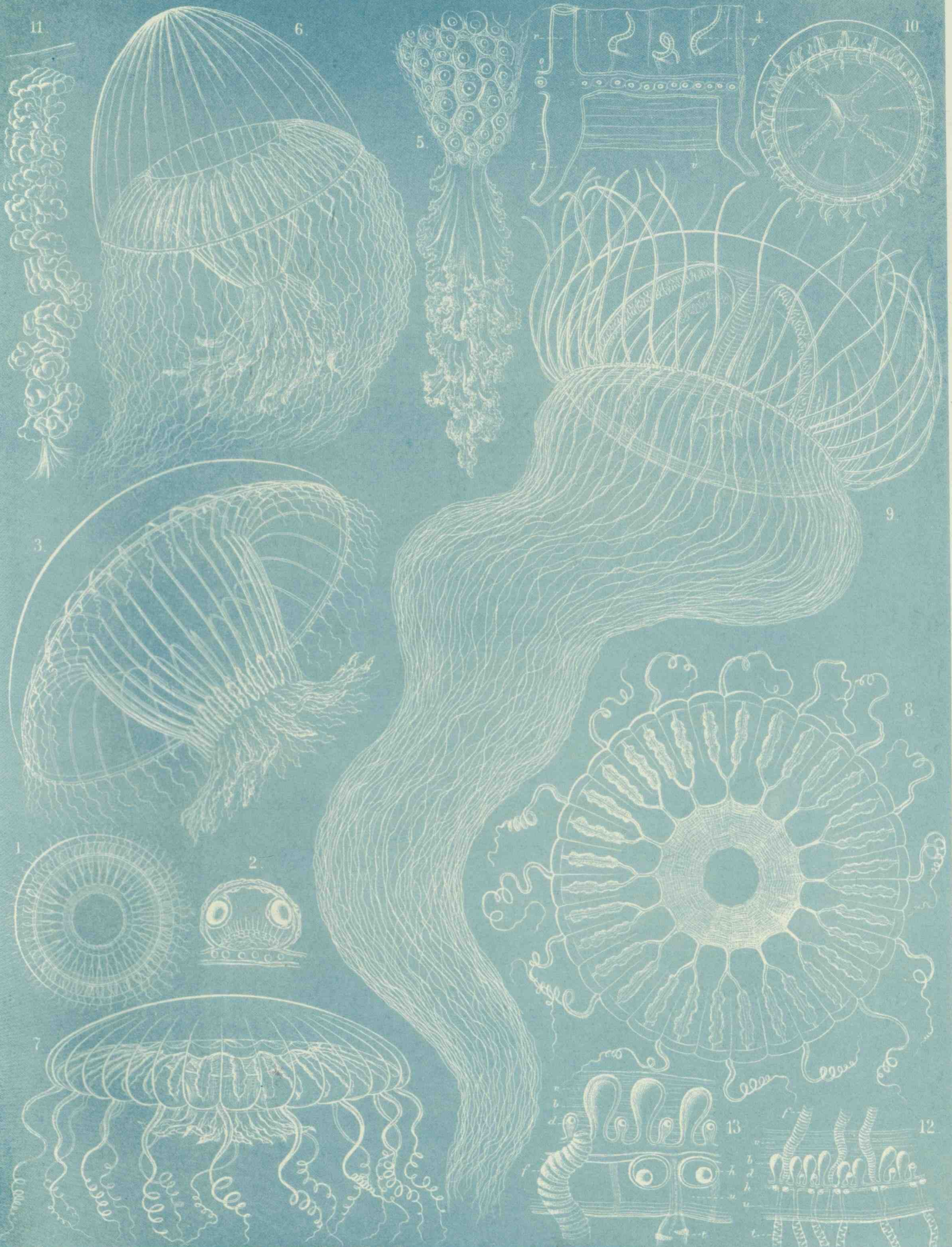
1. 2. Aequorea, 3-5. Orchistoma, 6-8. Zycocanna, 9-13. Olindias.
