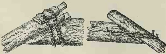
SECTION OF THE BRIDGE, SHOWING METHOD OF CONSTRUCTION.
