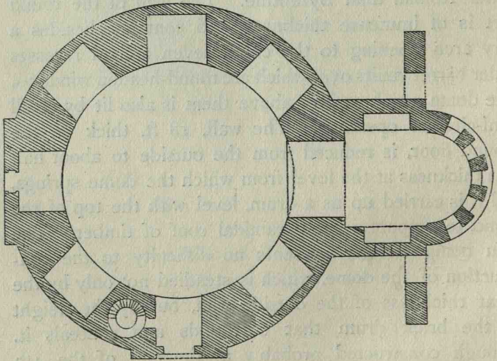
GROUND PLAN
