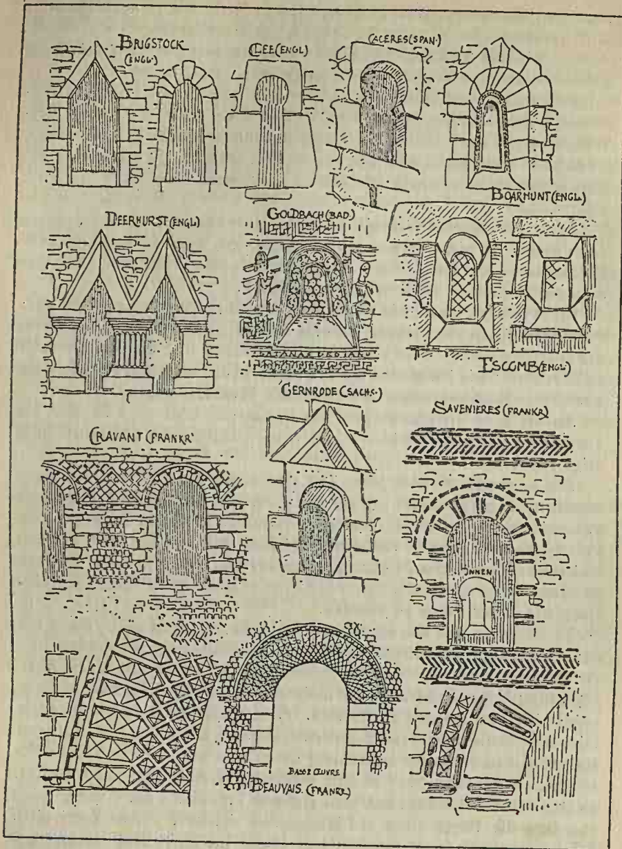
Abb. 60. Fensterformen.
