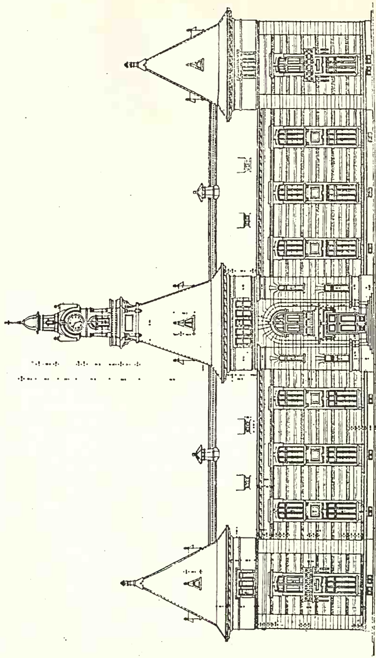
FATADA PRINCIPALA
